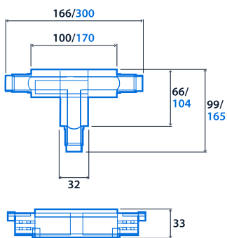
Tee Feed/Coupler
