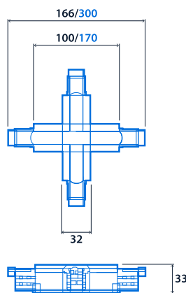
Cross feed
