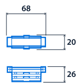
Straight Coupler
