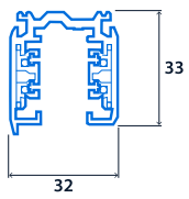
3-Circuit Track
