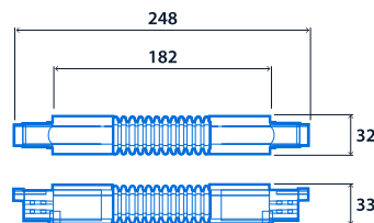
Flexible Coupler
