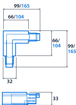
Angled Feed/Coupler
