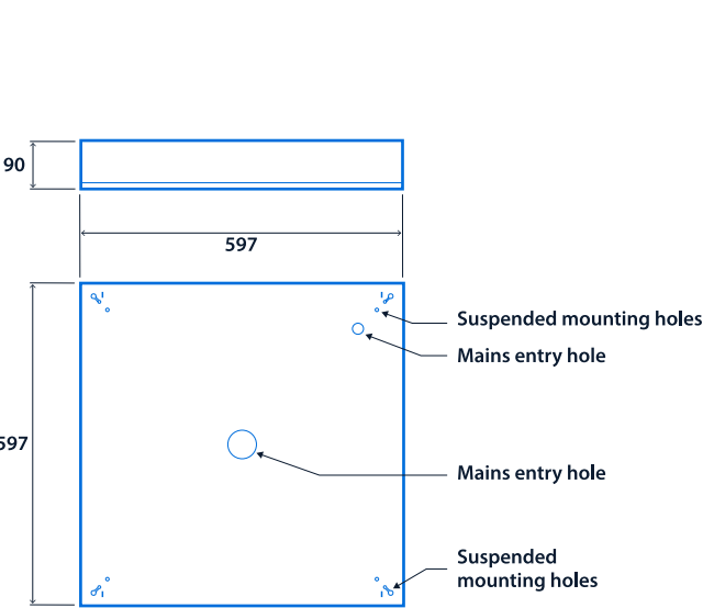
Surface/Suspended version 600 x 600
