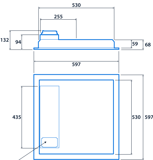
Recessed version 600 x 600
