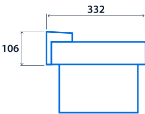
Cantilever Mounting
