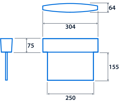
Ceiling Mounting
