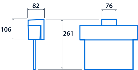
Wall Mounting
