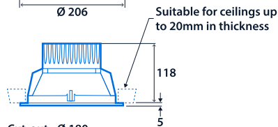
Cut-out - Ø 180 Minimum void depth - 200
